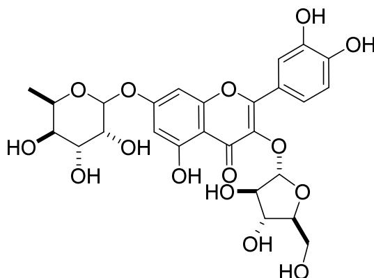
Kaempferol 3-O- \alpha -L-arabinofuranoside-7-O- \beta -D-rhamnoside (14).
