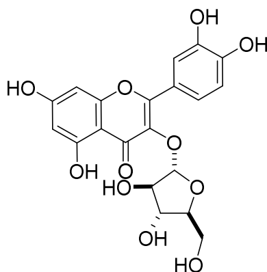
Quercetin 3-O- \alpha -L-arabinofuranoside (avicularine) (13).
