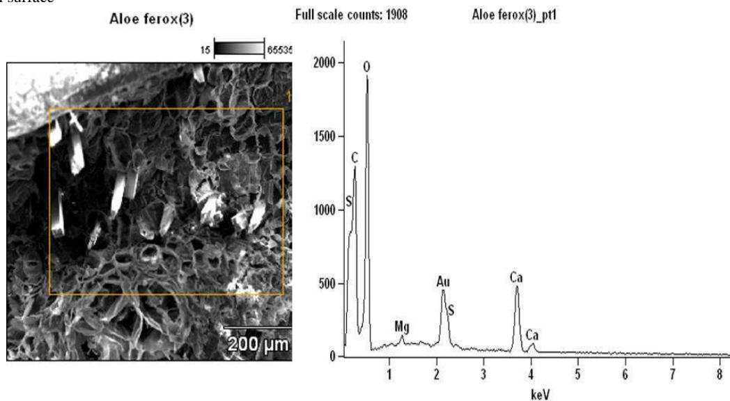
Figure 9: X-ray spectrum of mineral crystals deposits in the mesophyll tissue
