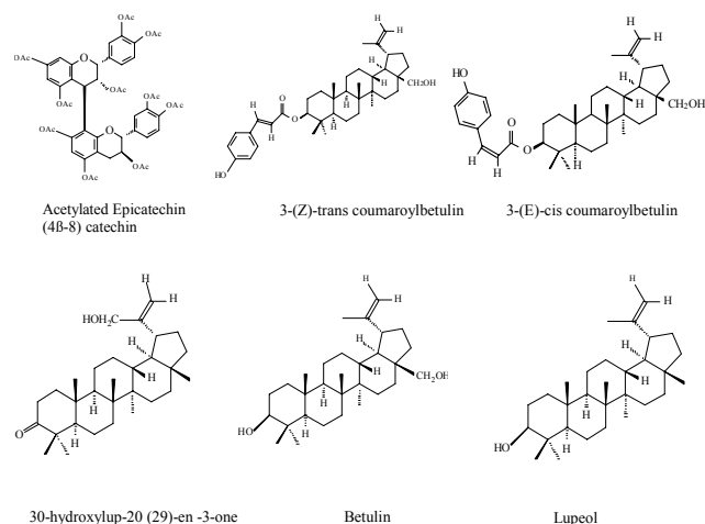
Figure 1: Isolated compounds
